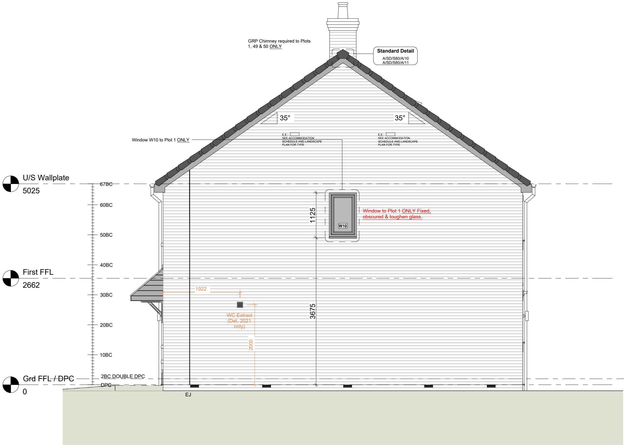
1 Gable Elevation 1 : 50
